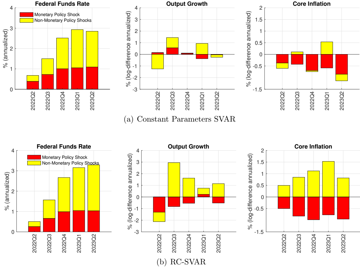
Figure 9: Monetary Policy vs Non-Monetary Policy Shocks
