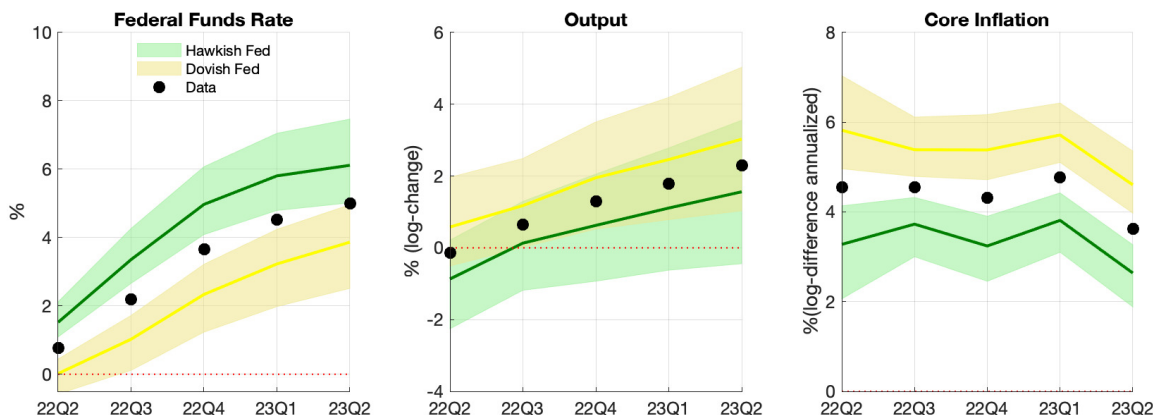
Figure 6: Counterfactuals Robust to Expectational Concerns
