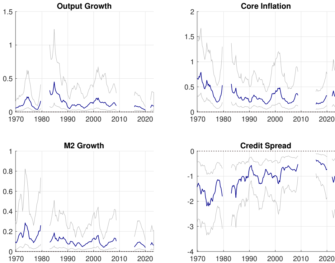
Figure 1: Contemporaneous Elasticities
