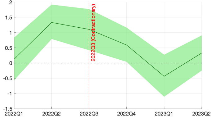
Figure 4: Monetary Policy Shocks
