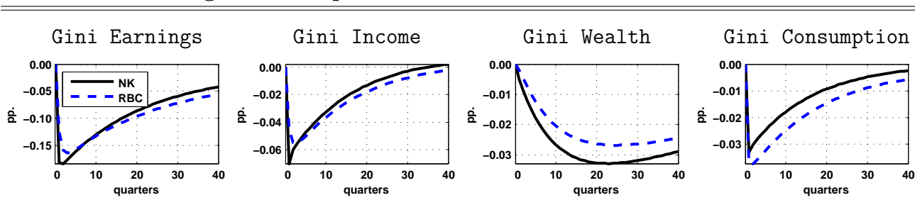
Figure 8: Response to a TFP Shock: Gini Indexes
