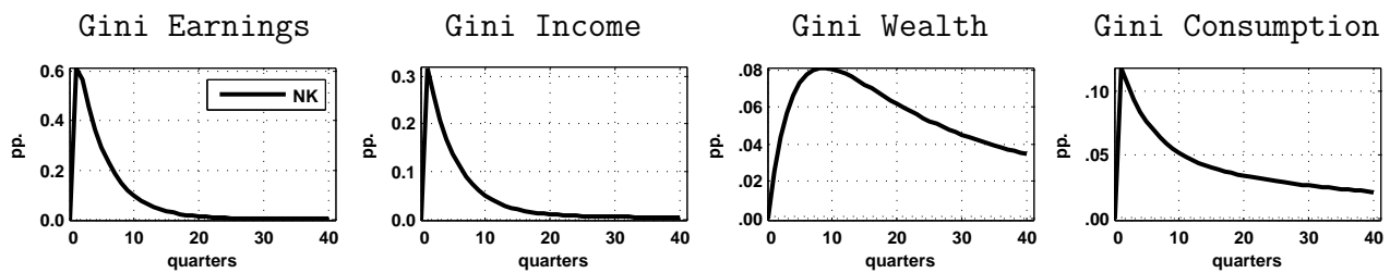
Figure 14: Response to a Monetary Policy Shock: Gini Indexes
