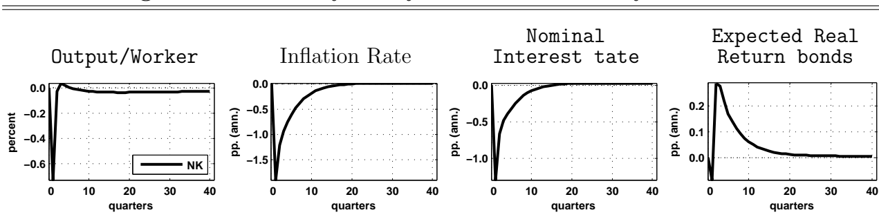
Figure 11: Monetary Policy Shock: Productivity and Prices
